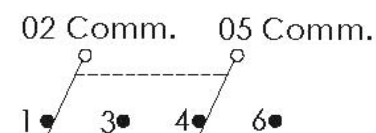
Schematic
