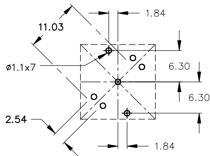
P.C. MOUNTING
