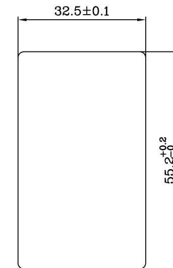
PANEL CUT-OUT
