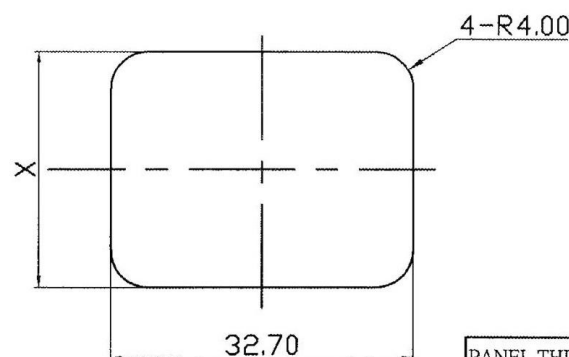
PANEL CUT-OUT
